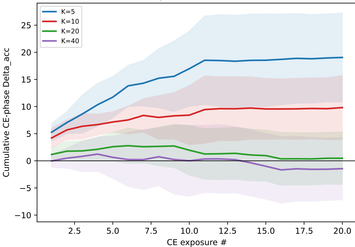
CE-pretrained teacher
