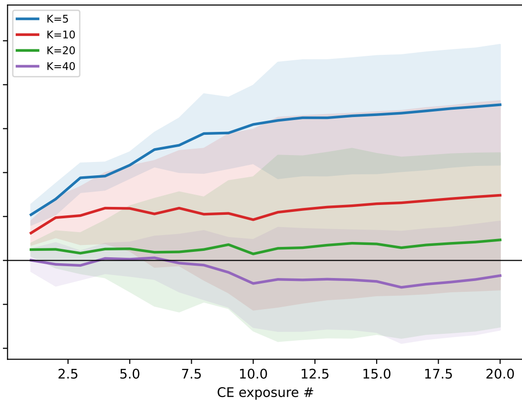
KL-self-distilled teacher
